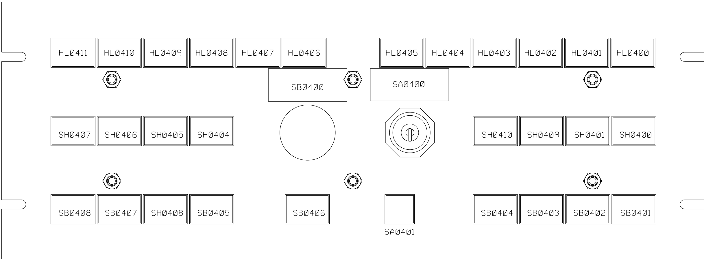
BACK VIEW WITH FLEX I/O REMOVED
