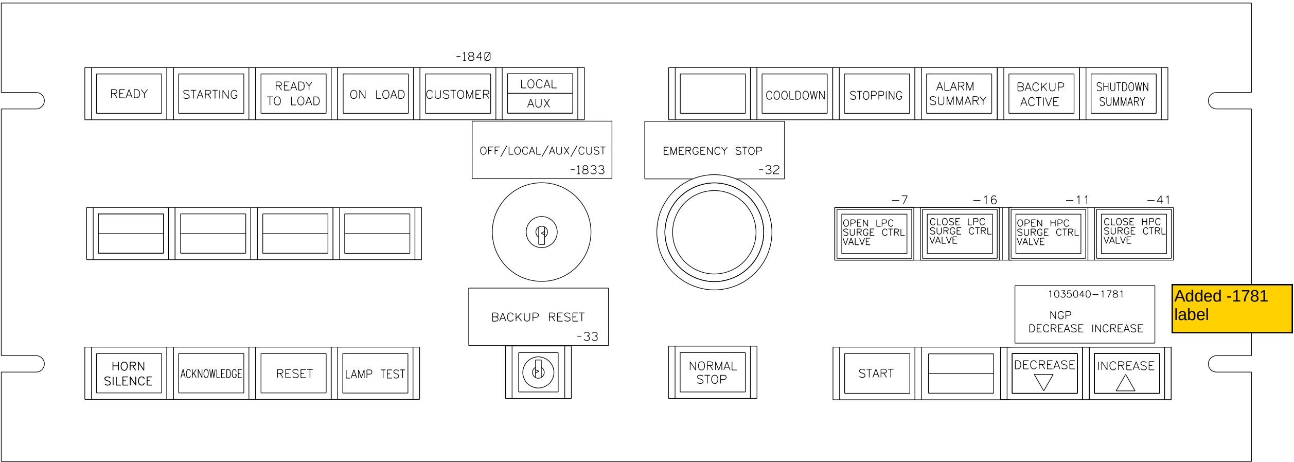
FRONT VIEW
